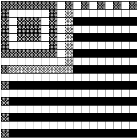
Mask Pattern 00
