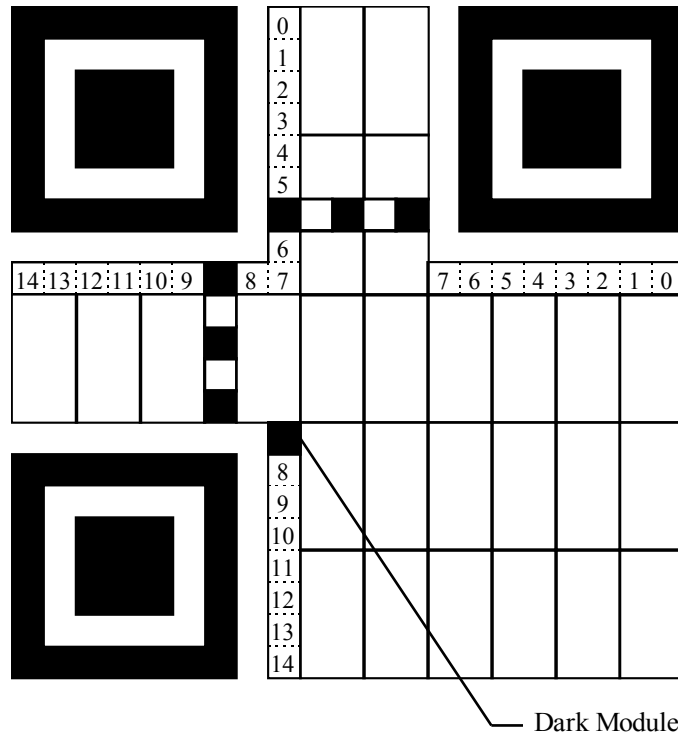
Figure 25 — Format information positioning
