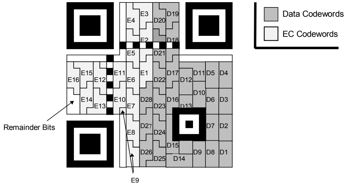
Figure 19 — Symbol character arrangement in version 2-M symbol
