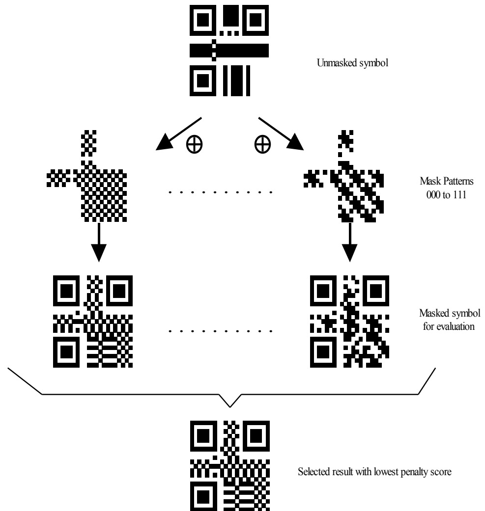
Figure 23 — Data masking simulation in QR Code symbols
