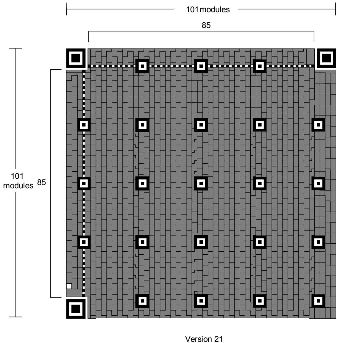
Figure 9 — Version 21 symbol
