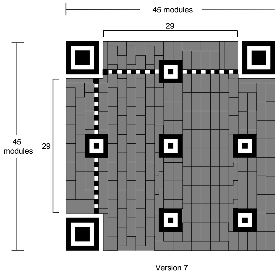
Figure 7 — Version 7 symbol
