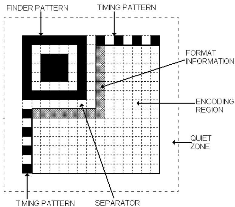
Figure 3 — Structure of a QR Code 2005 symbol
