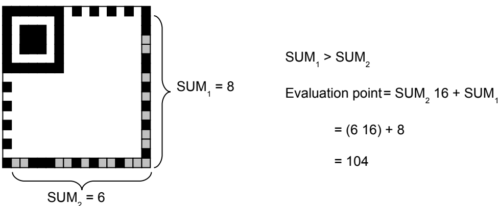
Figure 24 — Evaluation of masking results in Micro QR Code symbol
